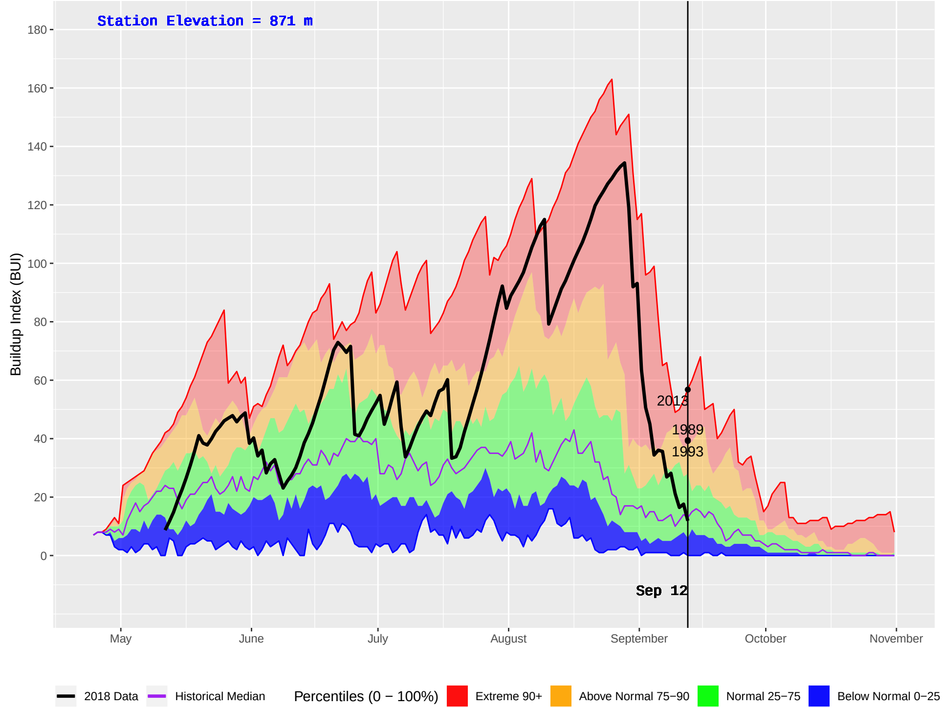
SUSTUT (156) : Historical (1989–2016) and Current (2018) Daily Buildup Index (BUI)
