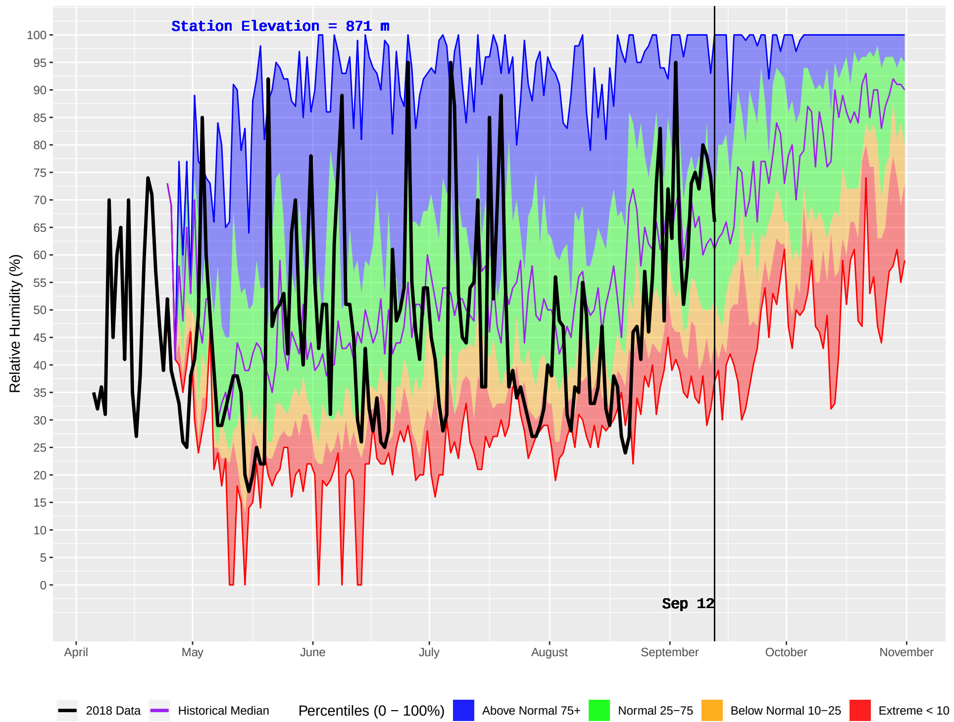
SUSTUT (156) : Historical (1989–2016) and Current (2018) Daily Relative Humidity
