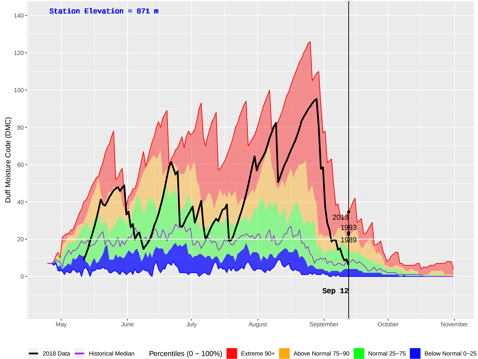
SUSTUT (156) : Historical (1989–2016) and Current (2018) Daily Duff Moisture Code (DMC)
