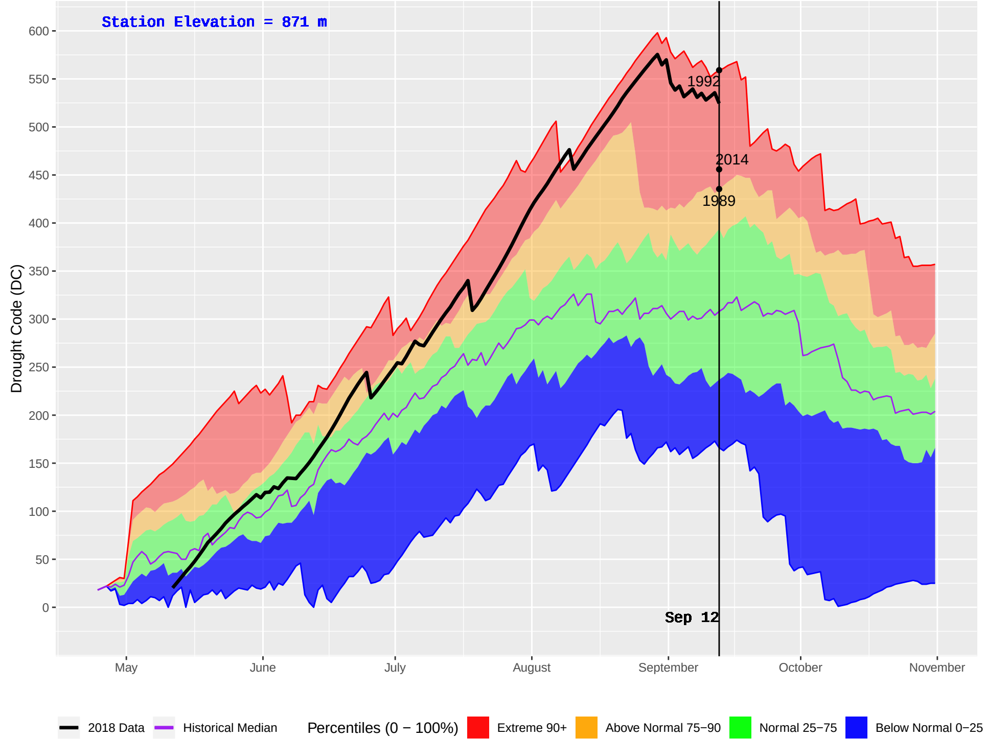
SUSTUT (156) : Historical (1989–2016) and Current (2018) Daily Drought Code (DC)
