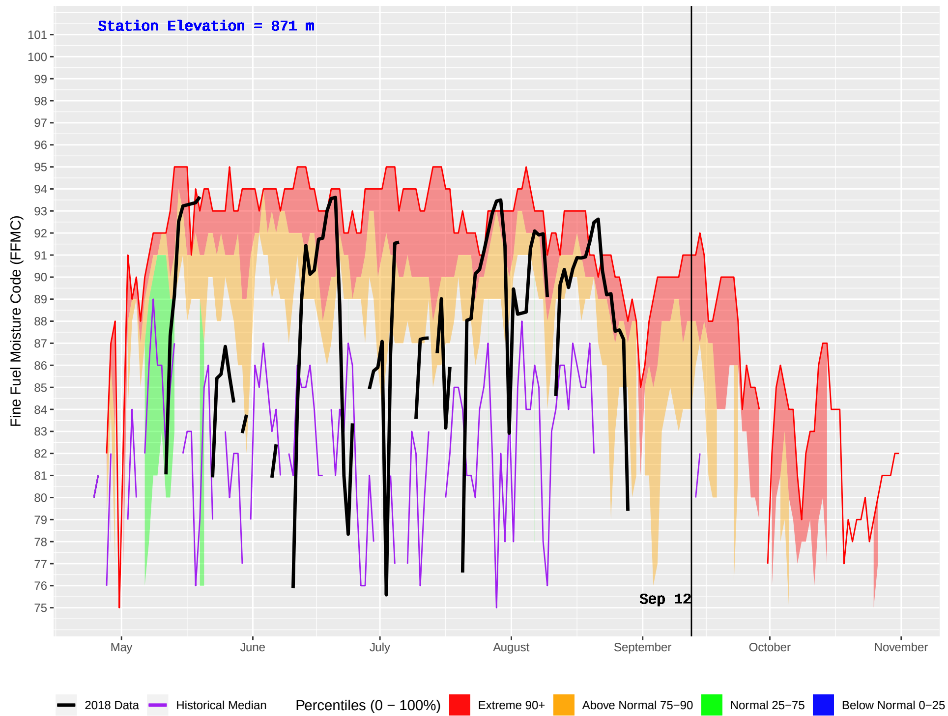
SUSTUT (156) : Historical (1989–2016) and Current (2018) Daily Fine Fuel Moisture Code (FFMC)
